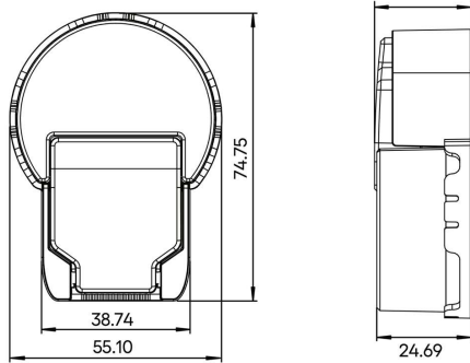
AIMO Relay 10A SK (550088) Dimensions in mm
