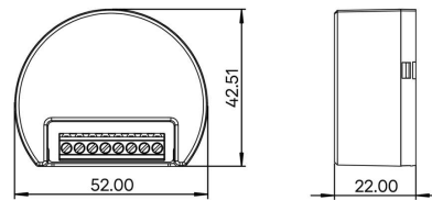
AIMO Relay 10A (550087) Dimensions in mm
